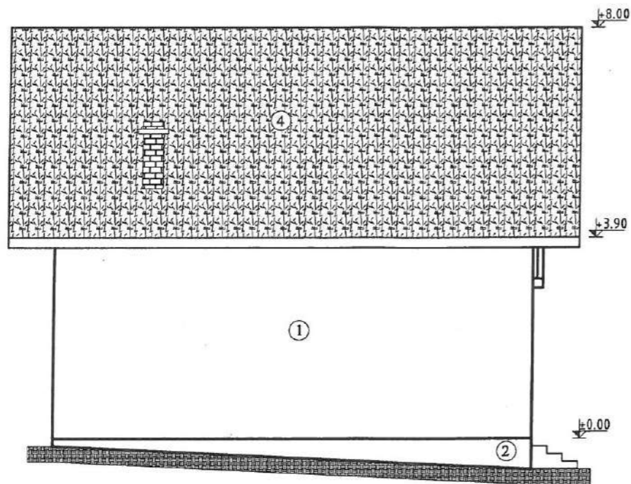
FATADA LATERALA B-B
