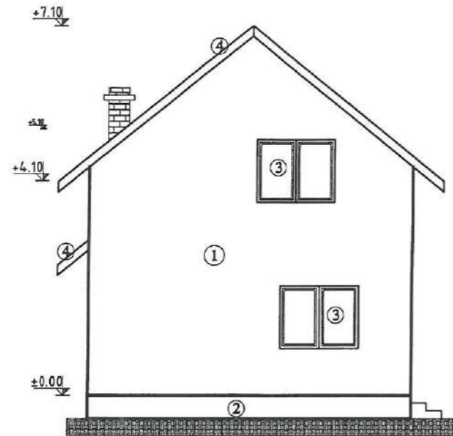
FATADA LATERALA B - B
