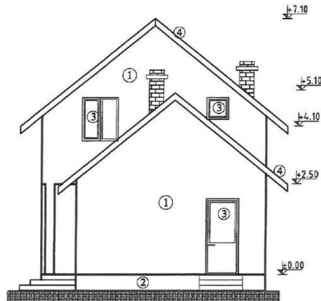
FATADA LATERALA D - D
